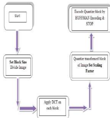
Fig. 3: Flow Chart for DCT Image Compression with Huffman Encoding
